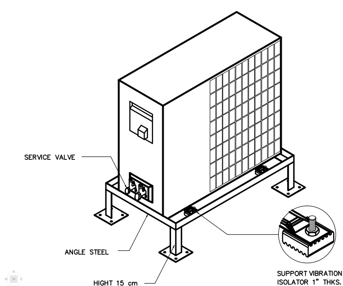
CONDENSING UNIT
