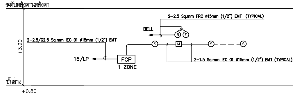
FIRE ALARM RISER DIAGRAM
