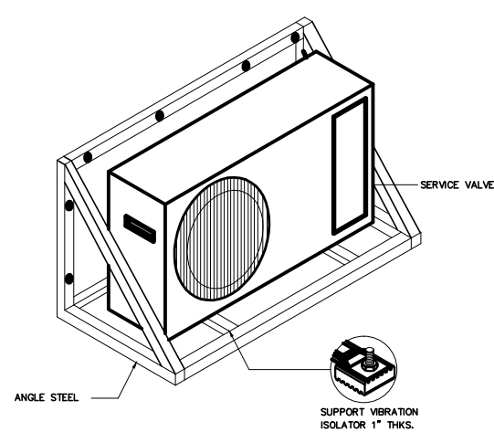
INSTALLATION OF CONDENSING UNIT
