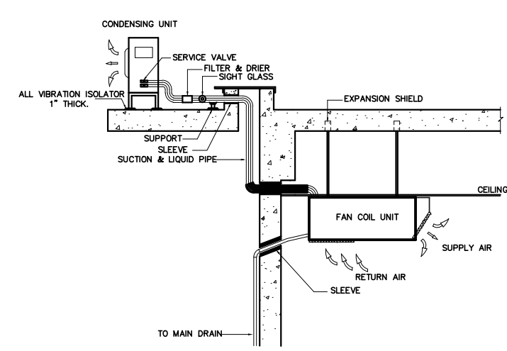
INSTALLATION OF AIR CONDITIONER (CEILING TYPE)
