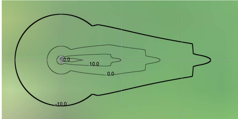
FIGURE 2 I/N Contours for IMT UE Interference into Fixed System A
