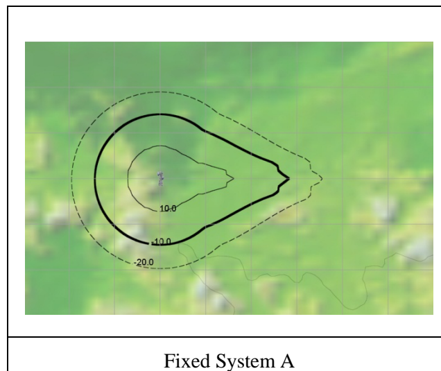
FIGURE 1 I/N contours for IMT base station interference into fixed systems A
