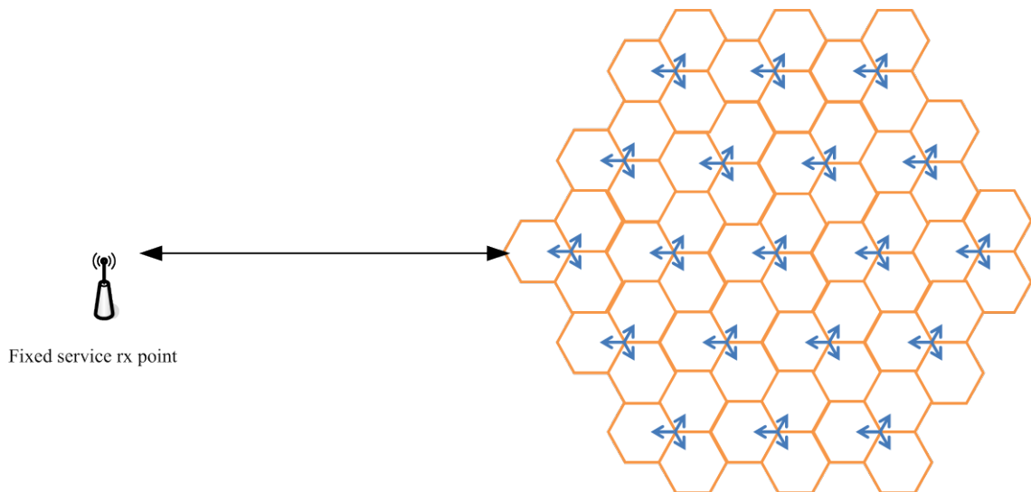
FIGURE 2 IMT macro cell scenario topology
