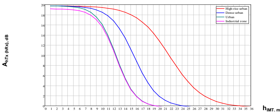
The additional loss due to protection from local clutter
