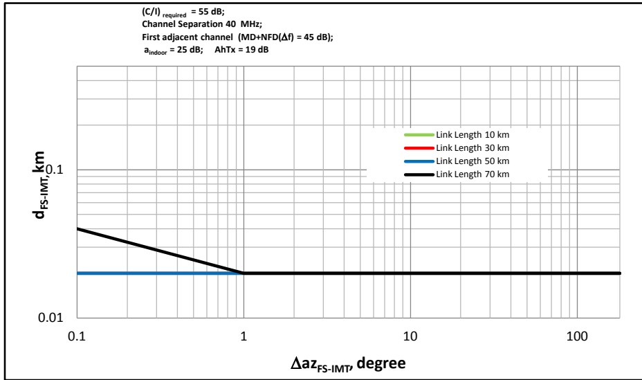
Required d_{\text{FS-IMT}} which is a function of angle \Delta az_{\text{FS-IMT}} (PP FS System type 1)
