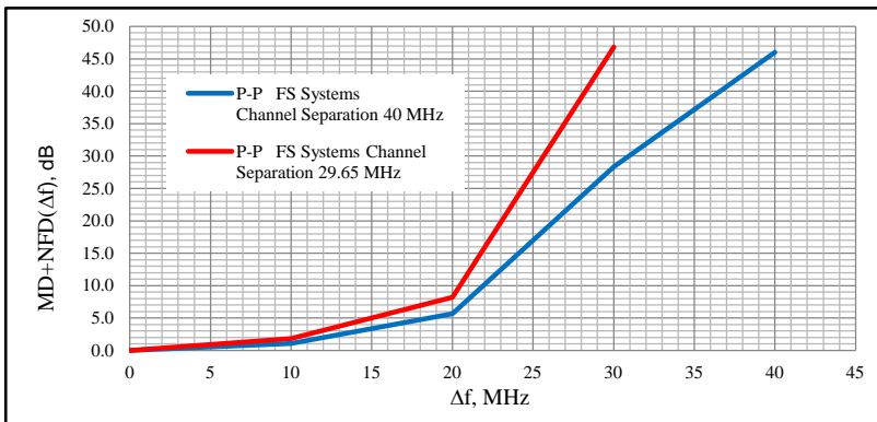
FIGURE 11 Attenuation (MD+NFD)
