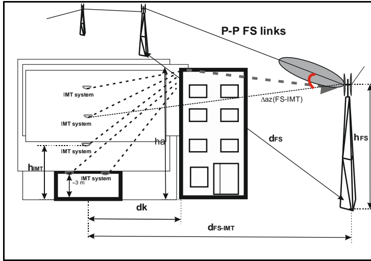
FIGURE 9 Urban interference scenario
