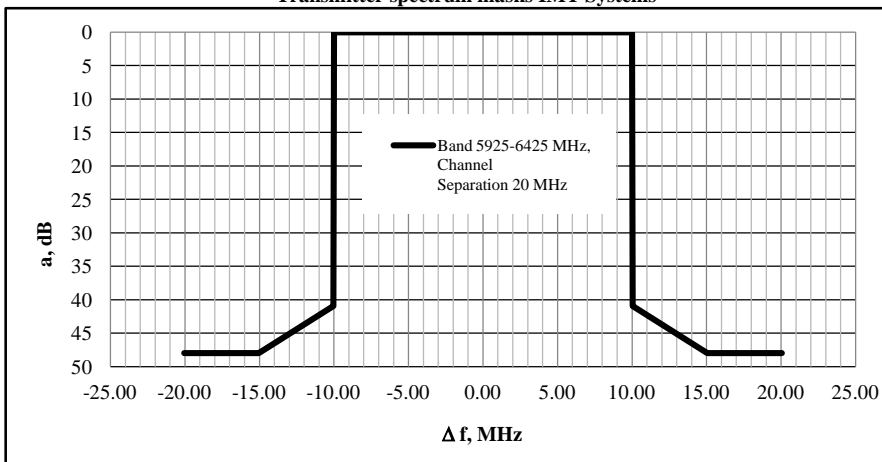
Transmitter spectrum masks IMT Systems
