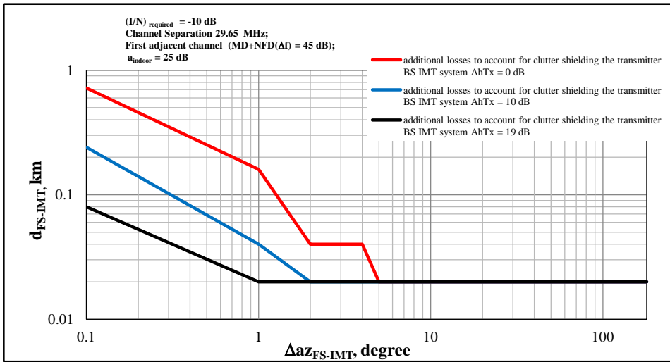
Required d_{FS-IMT} which is a function of angle \Delta_{az,FS-IMT} (PP FS System type 2)
