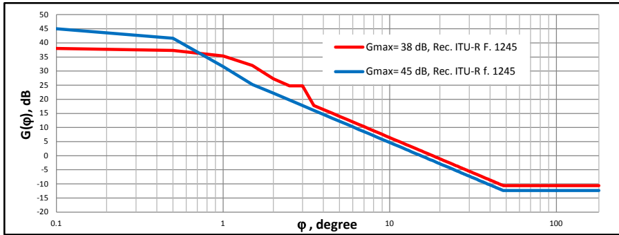
FIGURE 4 Antenna radiation pattern point-to-point FS system
